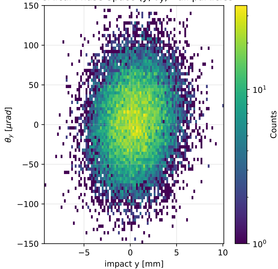
Vertical Phase Space (y, \theta_y ) - all particles
